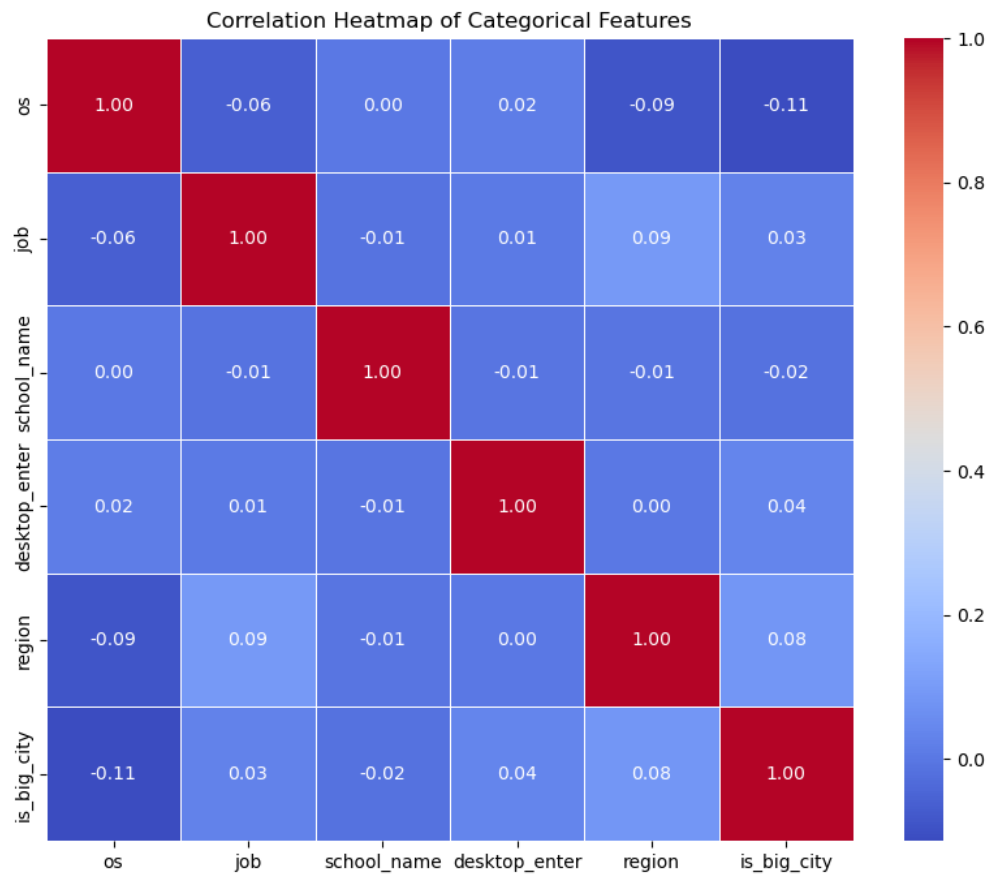
Figure 5 Correlation Heatmap of Categorical Features
