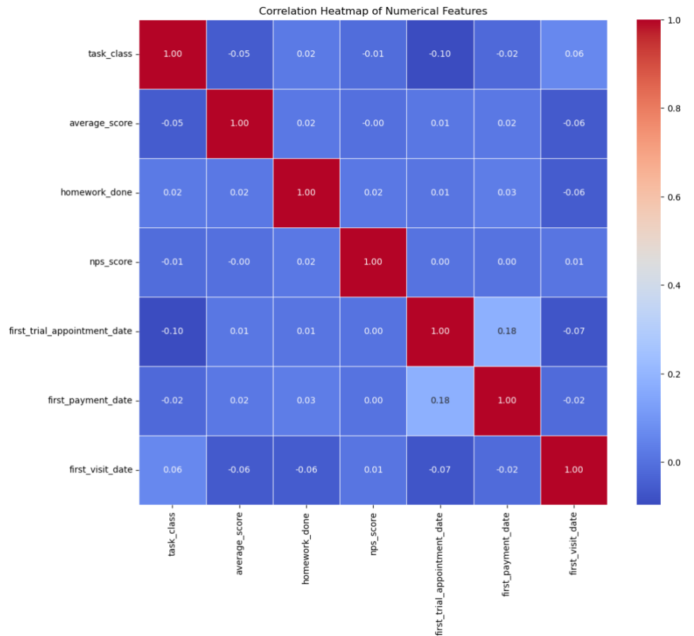
Figure 6 Correlation Heatmap of Numerical Features
